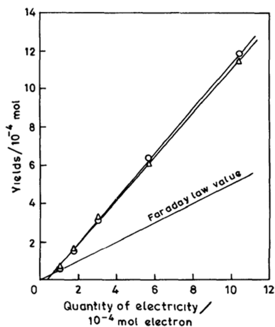
Figure 11. Variation of the yields of \text{H}_2 ( \circ ), and combined \text{H}_2\text{O}_2 (triangle) and \text{O}_2(^1\Delta) as a function of the charged transferred to the liquid during contact glow discharge electrolysis. Reproduced with permission from [238], copyright 1994 Elsevier.
