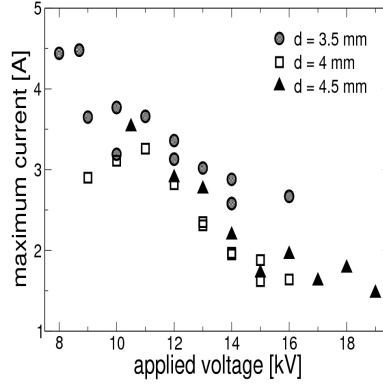
Fig. 6. Maximum current in pulse I_{max} as a function of applied voltage U_o .
