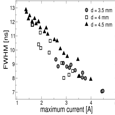
Fig. 7. Full width of the pulse at half maximum (FWHM) as a function of I_{max} .
