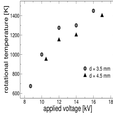
Fig. 8. Rotational temperature measured from N_2 (C-B, 0-0) as a function of U_o .
