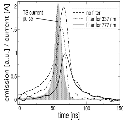
Fig. 10. Normalized temporal emission profiles obtained by PMT with filter for N_2 (C-B, 0-0) (337 nm), filter for O^* emission (777 nm), and with no filter.
