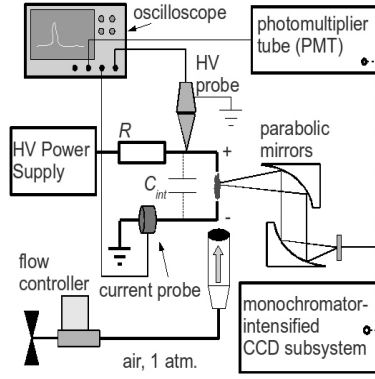
Fig. 1. Schematic of the experimental setup, HV – high voltage, R – resistor.
