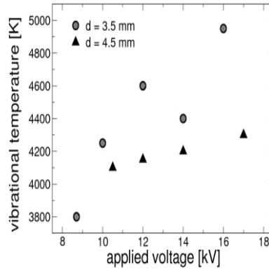
Fig. 9. Vibrational temperature of N_2 (C) species as a function of U_o .
