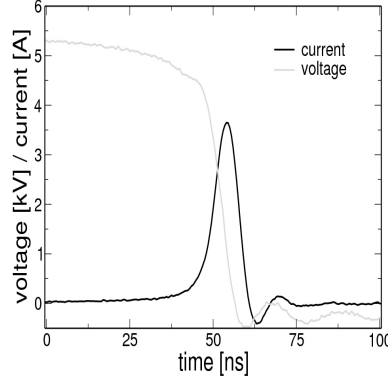
Fig. 2. Typical TS current and voltage waveforms, repetition frequency \sim 5 kHz, U_o = 10 kV.
