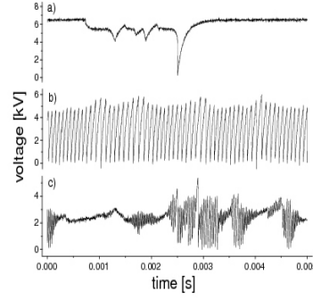
Fig. 3. Voltage waveforms of different discharge regimes: a) the first random TS pulses, b) regular TS, c) unstable glow regime.
