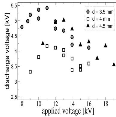
Fig. 5. Discharge voltage U_{TS} as a function of applied voltage U_o .
