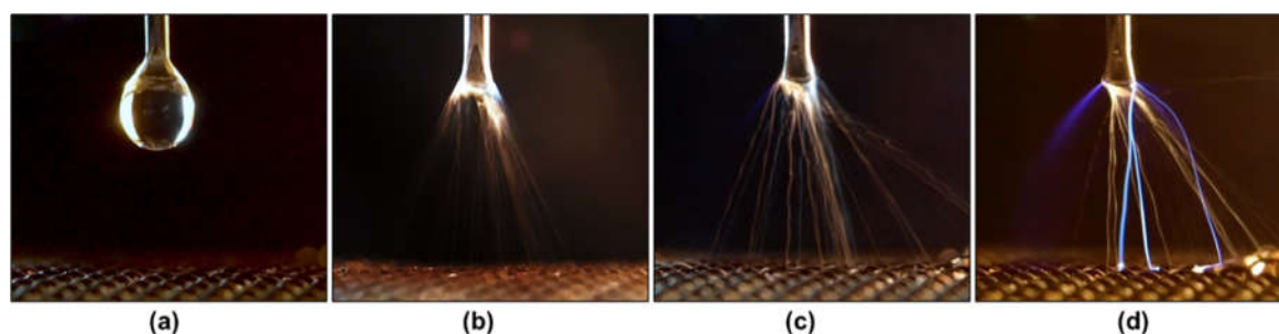
Figure 2. Photographs of the electrospaying of water in an 8-mm gap, water flow rate 0.5 \text{ mL min}^{-1} : (a) droplet without a high voltage, (b) electrospray with a high voltage applied, 5.5 kV, (c) electrospray combined with streamer corona, 6.5 kV, (d) electrospray with transition streamer corona-transient spark, 7.8 kV. Reproduced from Machala et al. [65]. All rights reserved.
