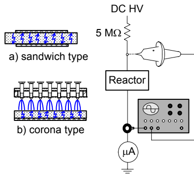
Fig. 1. Experimental apparatus.
