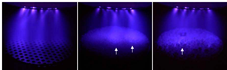
Fig. 13. Visual character of the discharge in corona geometry – materials: a) no dielectric, b) ceramic D, c) coating F, current: 400 \mu\text{A} , shutter speed: 8 s.
